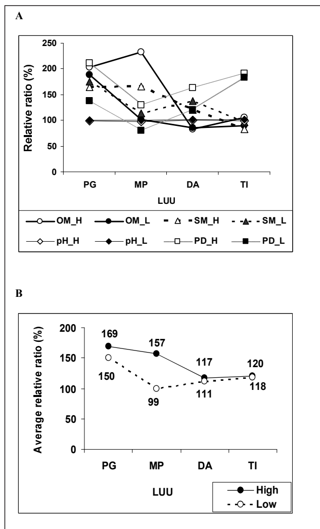
Figure 3: Soil properties relative ratio between each Land Use Units (LUU) and an adjacent national park (A), and average of the entire relative ratios for all soil properties for each LUU (B)
