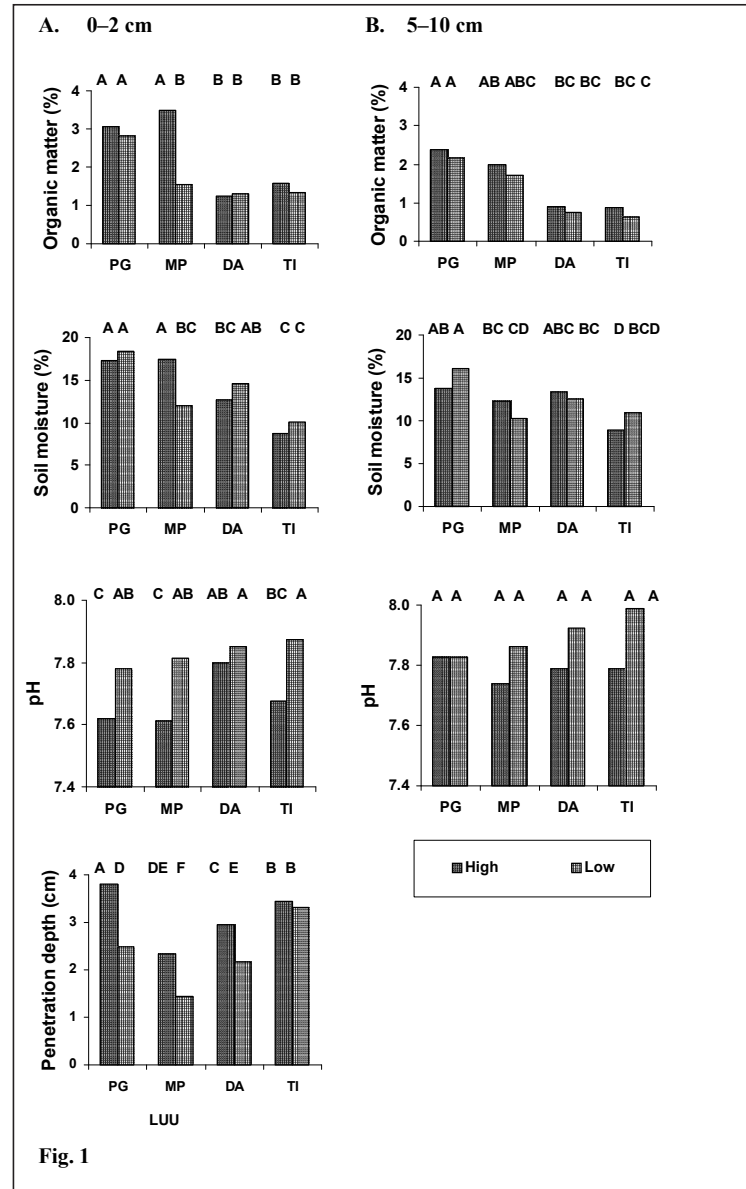
Figure 1: Averages of soil properties at different Land Use Units (LUU) in depths: 0–2 cm (A) and 5–10 cm (B)
