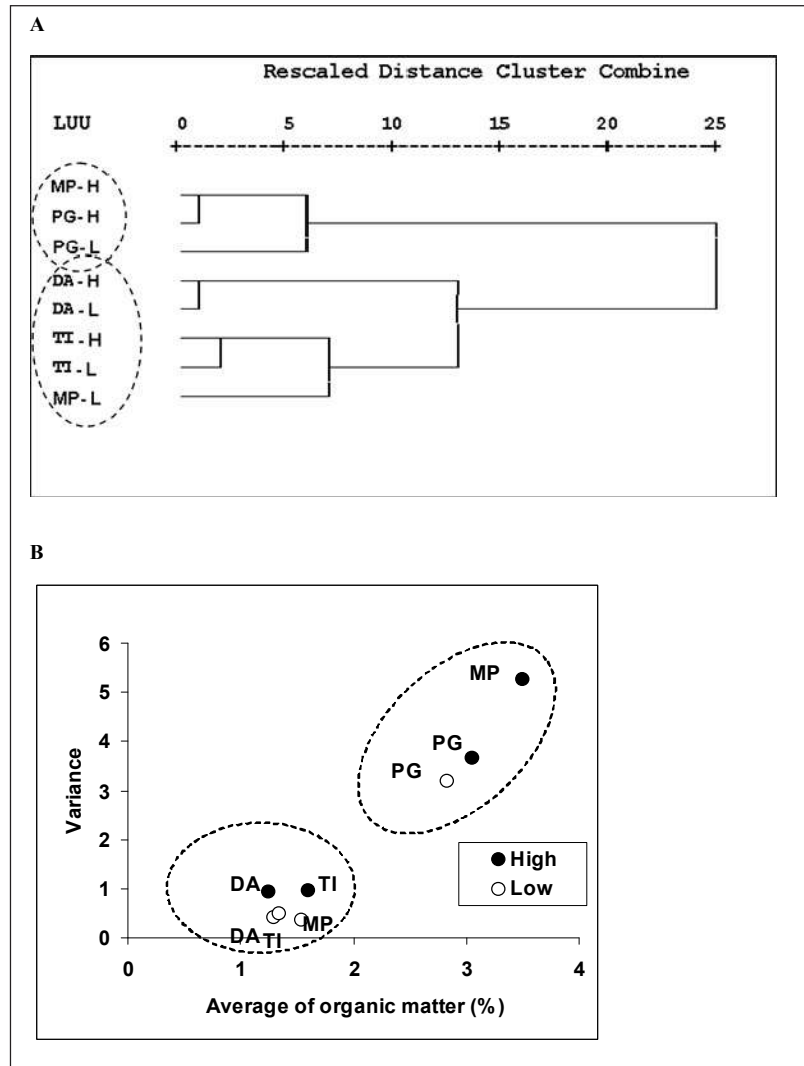
Figure 4: Dendrogram of hierarchical cluster analysis of urban Land Use Units (LUU) (Ward Method, using average linkage between groups) (A), and variance of organic matter as a function of the average at various LUU (B)
